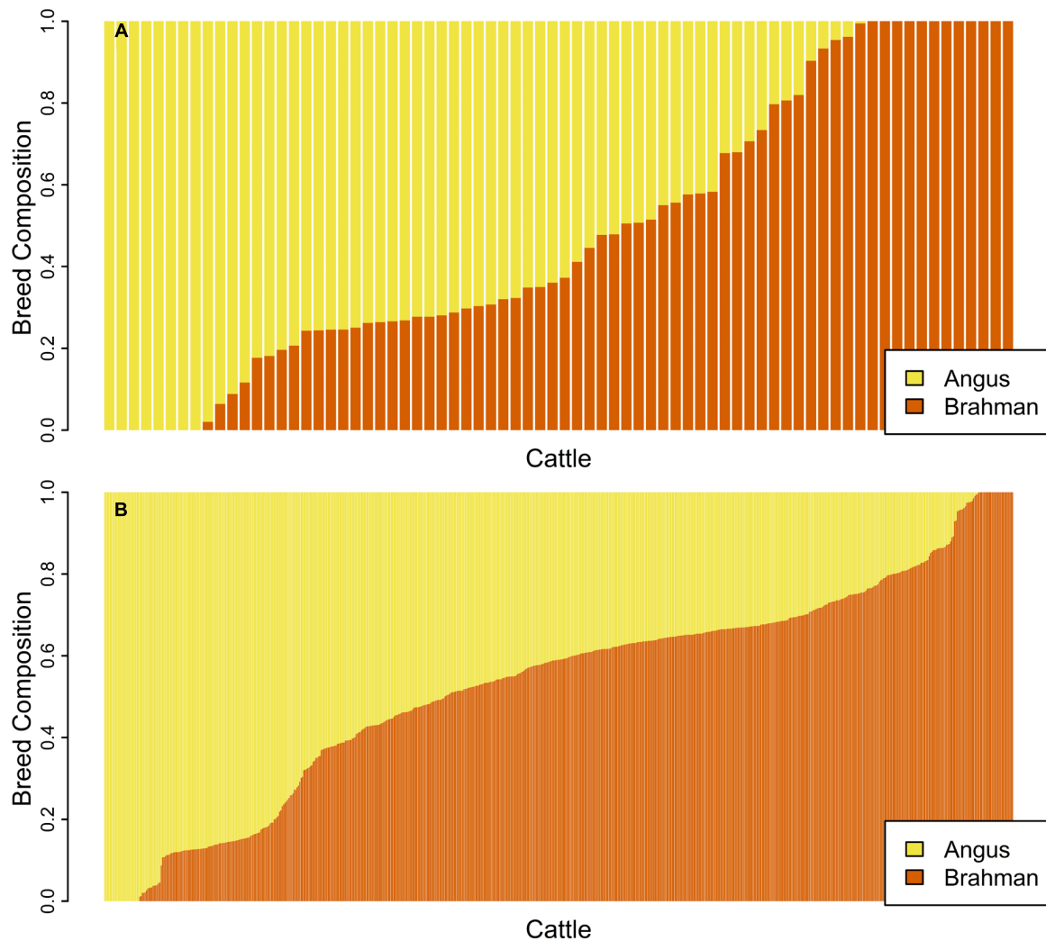
FIGURE 2 | Bar plot of the Q matrix from an unsupervised (A) ADMIXTURE run showing the proportion of the genome contributed by each breed for 74 unrelated samples. Panel (B) shows the Q matrix from a supervised run for 602 samples in the related set. Each vertical bar represents an individual with yellow showing the proportion of the genome with Angus ancestry and orange corresponds to the proportion of the genome with Brahman ancestry.
