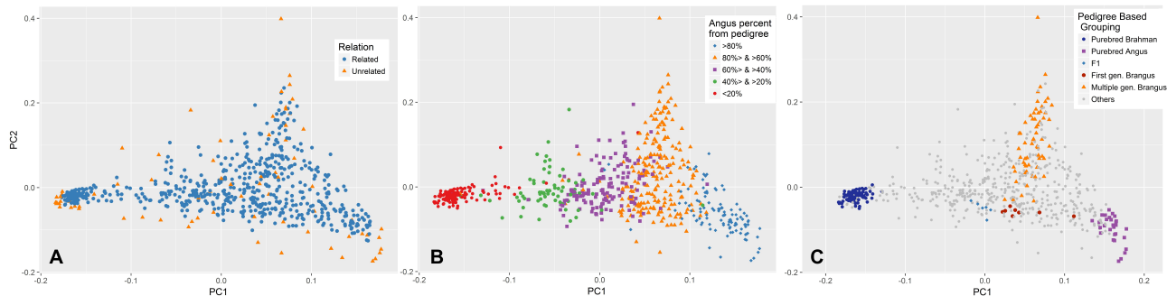
FIGURE 4 | Population distribution across the first (PC1) and second principal component (PC2). (A) PCA was performed on the unrelated set of animals (blue) and PC1 and PC2 values for the rest of animals (orange) were predicted based on their genetic similarity to animals in the unrelated set. (B) Animals are labeled based on their pedigree breed composition which can be described by the variation in PC1. (C) Brangus cattle from one or more generations of Brangus–Brangus matings show more scatter across PC2. In contrast, first generation Brangus and F1 cattle showed minimal scatter across PC2 and were close to the line connecting the two purebred clusters.
